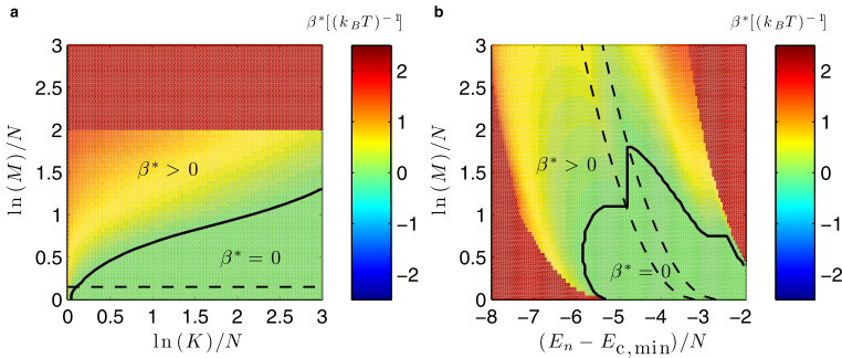
Fig. 4 Color representation of the dependence of the parameter \beta^* on the number of selected TCRs ( \ln(K)/N ), the number of self peptides ( \ln(M)/N ) against which TCRs were selected, and threshold for negative selection E_n/N . Parameters are: (E_p - E_n)/N = 0.5 \text{ k}_B \text{ T} and E_{c,\text{min}} - E_{c,\text{max}} = E_n - E_p , in the limit of large N . Solid black lines separate regions with \beta^* > 0 and \beta^* = 0 . The regions below the black dashed line in (a) and between the black dashed lines in (b) correspond to \beta = 0 (every TCR is selected). In (a) E_{c,\text{min}} = E_n - N\bar{J} and in (b) \ln(K)/N = 1.5
