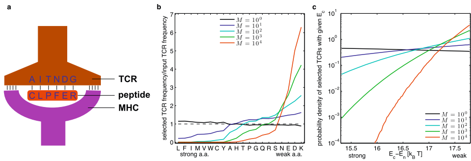
Fig. 1 Effects of thymic selection on the characteristics of selected TCRs. (a) Schematic representation of the interface between TCR and pMHCs. The region of the TCR contacting the peptide is highly variable and is modeled by strings of amino acids of length N . The peptide is also treated similarly. The binding free energy between the TCR and the entire pMHC is computed as described in the text. (b) Amino acid composition of TCR selected against M types of self peptides in the thymus. The ordinate is the ratio of the frequency of occurrence of an amino acid in the peptide contact residues of selected TCRs and the pre-selection frequency. TCRs selected against many types of self-peptides in the thymus have peptide contact residues that are enriched in amino acids that interact weakly with other amino acids. Amino acids on the abscissa are ordered according to their largest interaction strength with other amino acids in the potential matrix, J . (c) Probability density distribution of E_c values (strength of TCR binding to MHC) of TCRs selected against M types of self peptides. TCRs selected against many types of self peptides are more likely to bind weakly to MHC. The parameter values are: N = 5 , E_p - E_n = 2.5 \text{ k}_B T , E_{c, \max} = E_p - N\bar{J} , E_{c, \min} = E_n - N\bar{J} . We have used the Miyazawa-Jernigan matrix, J [21] and amino acid frequencies f_a from the human proteome [11, 17] (using the mouse proteome does not change the qualitative results [17])
