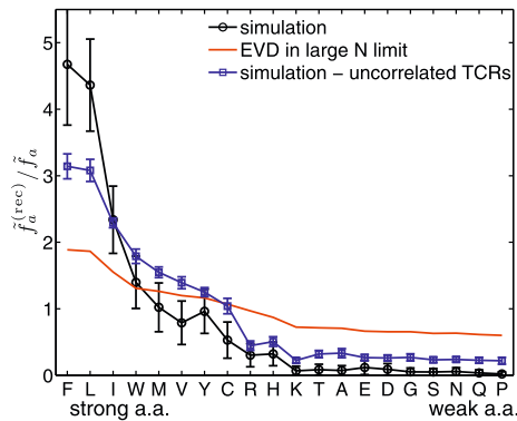
Fig. 5 Amino-acid composition of recognized foreign peptides. The amino acids are ordered in decreasing frequency along the abscissa. The data points in black are obtained numerically with the parameters relevant to TCR selection in the mouse and K = 10^3 TCRs, which were then challenged with L. monocytogenes peptides (see text). The blue data points are for similarly challenged K = 10^3 uncorrelated TCRs. The error bars reflect the sample size used to generate the histograms and differences for different realizations of M self peptides (black) or K uncorrelated TCRs (blue). The red line is the result of the EVD analysis in the large N limit from (15), where TCR amino acid frequencies were obtained from (9). In all cases we have used the Miyazawa-Jernigan matrix, J [21], amino acid frequencies f_a from the human proteome (using the mouse proteome does not change the qualitative results [17]), and amino acid frequencies \bar{f}_a from the L. monocytogenes proteome [11, 17]
