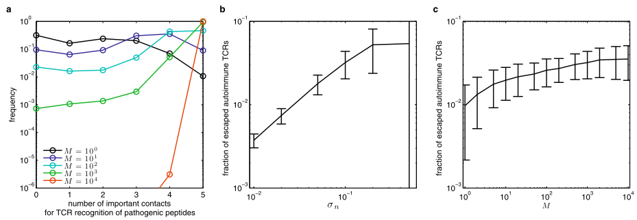
Fig. 7 Thymic selection with soft thresholds for positive and negative selection. (a) Histogram of the number of important contacts (defined in text) with which T cells recognize pathogenic peptides. This result and other characteristics of selected TCRs (data not shown) are qualitatively equivalent to the results obtained with sharp thresholds for positive and negative selection (Figs. 1 and 3). (b) Fraction of escaped autoimmune TCRs (ratio of the numbers of escaped autoimmune TCRs to selected TCRs) as a function of the softness of the threshold for negative selection \sigma_n . Fraction of autoimmune TCRs increases with \sigma_n , until the softness of the thresholds becomes of the same order as the separation between the thresholds of positive negative selection, \sigma_n + \sigma_p \sim E_p - E_n . \sigma_p = 1 \text{ k}_B \text{ T} , M = 10^3 . (c) Fraction of escaped autoimmune TCRs as a function of the number of types of self peptides ( M ). Fraction of autoimmune TCRs increases with M and is roughly constant for large M , however the absolute numbers of TCRs are decreasing with M . \sigma_p = 1 \text{ k}_B \text{ T} , \sigma_n = 0.1 \text{ k}_B \text{ T} . The error bars in (a) and (b) correspond to the standard deviation of the fractions of escaped TCRs obtained from repeating the thymic selection process many times
