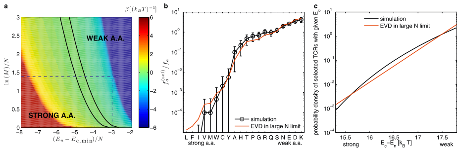
Fig. 2 Analytical results for characteristics of selected TCRs. (a) Representation of the dependency of the parameter \beta (a measure of amino acid composition of selected TCRs and a measure of selected TCR binding strengths to MHCs, see text), on the number of self-peptides ( \ln M/N ) and the threshold for negative selection E_n with (E_p - E_n)/N = (E_{c,max} - E_{c,min})/N = 0.5 \text{ k}_B \text{ T} . The region between the black lines corresponds to \beta = 0 , to the right (left) of which negative (positive) selection is dominant, and weak (strong) amino acids are selected. The blue dashed lines indicate the relevant parameter values for thymic selection in mouse. (b) Amino-acid composition of selected TCR sequences, ordered in increasing frequency along the abscissa. (c) Probability density distribution of E_c values (strength of TCR binding to MHC) of selected TCRs. (b–c) The data points in black are obtained numerically with the parameters relevant to mouse (see text). The error bars reflect the sample size used to generate the histograms and differences for different realizations of M self-peptides. The red lines are the result of the EVD analysis in the large N limit (from (9) and (10)), and the agreement is quite good. In both cases we have used the Miyazawa-Jernigan matrix, J [21] and amino acid frequencies f_a from the human proteome [11, 17]
