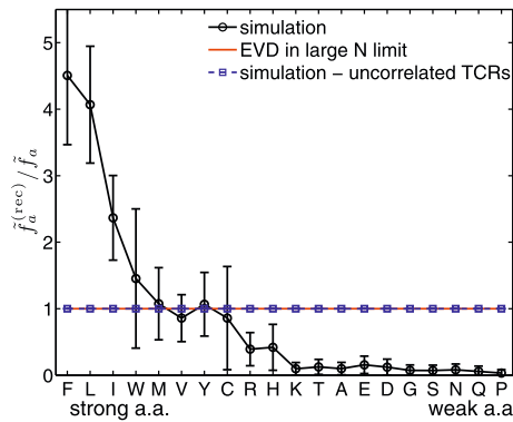
Fig. 6 Amino-acid composition of foreign peptides recognized by a complete pool of selected TCRs. The amino acids are ordered in decreasing frequency along the abscissa. The data points in black are obtained numerically where a complete pool of selected TCRs (obtained from thymic selection of all 20^N TCR sequences against M = 10^3 self peptides) is challenged with L. monocytogenes peptides (see text). The error bars reflect the differences for different realizations of M = 10^3 self peptides. The red line is the result of the EVD analysis in the large N limit from (20). The data points in blue are obtained numerically where a complete pool of uncorrelated TCRs, which is equal to the complete pool of 20^N sequences (see text), are challenged with L. monocytogenes peptides. In this case, there are no error bars, because we use the complete pools of TCRs and foreign peptides with appropriate weights. In all cases we have used the Miyazawa-Jernigan matrix, J [21], amino acid frequencies f_a from humans (using the mouse proteome does not change the qualitative results [17]), and amino acid frequencies \hat{f}_a from the L. monocytogenes [11, 17]
