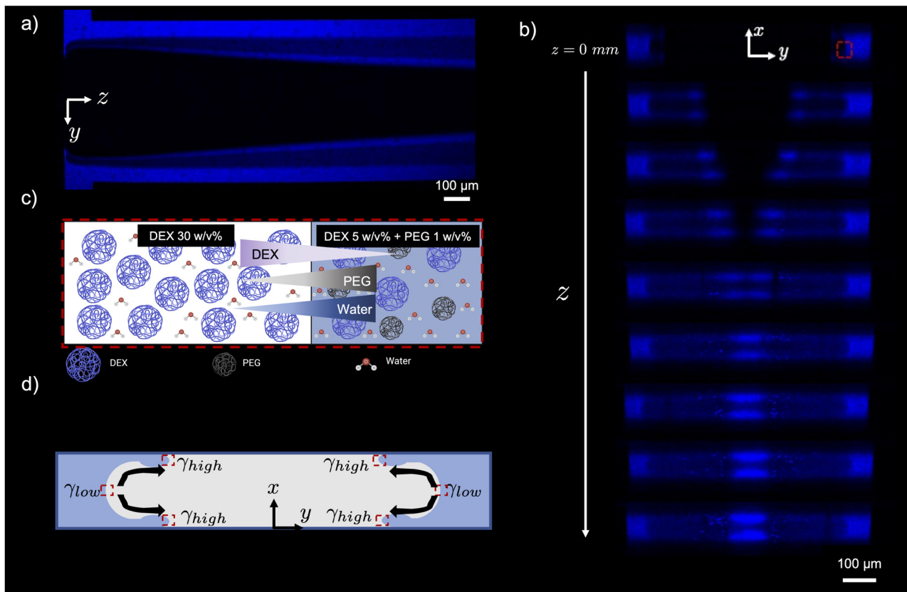
Fig. 2 (a) Fluorescent image of the y - z view of the flow-focusing junction of the microchannel at x \approx 0 (the bottom of the channel), after the system reaches steady-state, where the inner stream of DEX 30 w/v% (not visualized) is surrounded by a miscible solution of DEX 5 w/v% and PEG 1 w/v% (doped with Alexa Fluor dye). Two fronts can be seen moving towards the center of the channel. (b) Steady-state confocal microscopy images showing flow cross sections every 1 mm downstream along the z direction. Upstream, moving fronts from the outer streams are formed on both top and bottom walls of the device. The fronts move towards the center of the channel further along z , and at about z \approx 5 mm they merge, resulting in formation of a central fluid thread on the top and bottom walls. (c) Illustration of species within the system at early times within the red rectangle shown in (b), near the diffuse boundary between solutions 1 and 2. The image is created with ( https://www.biorender.com ). The concentrations of species are set such that water will be withdrawn from the outer stream towards the inner stream, and should be faster near the walls due to weaker effects of convection (no-slip condition). This schematic indicates the relative concentration of species across the two fluid streams, and does not provide any insight on the conformation and polymer chain morphology in the solution. (d) Schematic of the channel cross section illustrating the proposed mechanism for the advancement of the fronts. The withdrawal of water from the outer stream towards the inner stream near the walls results in an increase of polymer concentrations and therefore induces phase separation and nucleation of a PEG-rich zone near the interface. Due to the concentration gradient present across the interface between the two streams, a gradient in tension \nabla\gamma induces Marangoni flow, causing the PEG-rich zone to move towards the center of the channel, forming fronts on both top and bottom walls, with the original nucleated PEG-rich zone being the tip of these moving fronts.
