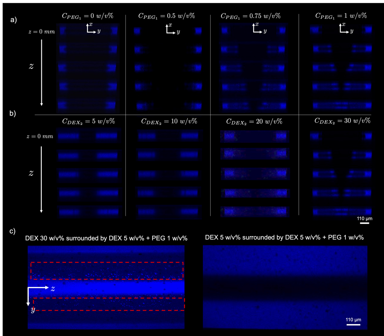
Fig. 3 Confocal microscopy scans in the x - y plane, taken every 1 mm downstream in z , for different systems where (a) C_{PEG_1} is varied from 0, 0.5, 0.75 and 1 w/v% while keeping C_{DEX_1} = 5 w/v% and C_{DEX_2} = 30 w/v% and (b) C_{DEX_2} is varied from 5, 10, 20 and 30 w/v% while keeping C_{DEX_1} = 5 w/v% and C_{PEG_1} = 1 w/v%, with all experiments set with Q_1 = 2 \mu\text{L min}^{-1} and Q_2 = 1 \mu\text{L min}^{-1} . As seen in panel a, With C_{PEG_1} of 0 and 0.5 w/v%, after the flow reaches steady-state, invasion fronts are not formed. Instead, we observe that the Alexa Fluor dye diffuses from the outer streams towards the center of the channel. With no PEG in the system or a low C_{PEG_1} = 0.5 w/v%, the initial concentration of the system is set within the miscible regime, therefore no liquid-liquid phase separation occurs. As C_{PEG_1} is increased to 0.75 and 1 w/v%, the system undergoes liquid-liquid phase separation and invasion fronts can be seen moving towards the center of the channel. Similarly, for experiments where C_{DEX_2} is tuned (as shown in panel b), lower C_{DEX_2} of 5 and 10 w/v% do not exhibit an advancing front, since the flow system is fully miscible. However, for higher concentration of C_{DEX_2} of 20 or 30 w/v%, the system becomes susceptible to liquid-liquid phase separation, therefore triggering nucleation of a PEG-rich phase near the interface and then formation of a PEG-rich moving front due to a gradient in tension present across the width of the front. (c) Fluorescent flow images in the y - z plane at x \approx 50 \mu\text{m} (at the top wall of the channel) and z ranging from 5 mm to 6.5 mm, for system of DEX 30 w/v% surrounded by miscible solution of DEX 5 w/v% and PEG 1 w/v% (left image) and DEX 5 w/v% surrounded by miscible solution of DEX 5 w/v% and PEG 1 w/v% (right image). PEG-rich droplets can be seen flowing parallel to the nucleated PEG film on the top wall (within the dashed red box in the left image), while no trace of phase separation can be seen in the system DEX 5 w/v% as the inner stream (right image).
