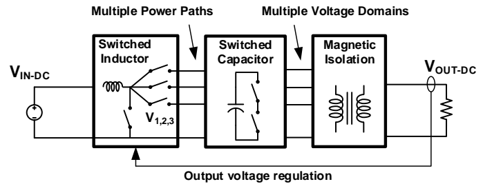
Fig. 2. Block diagram of a Multitrack dc-dc architecture [1].
