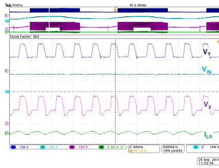
Fig. 20. ZVS waveforms with 250V AC input and 12V DC output at 100W.
