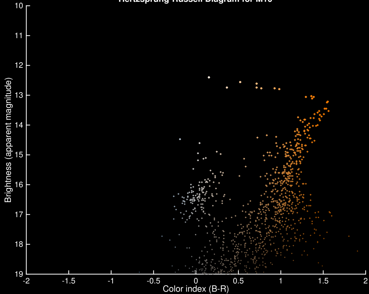
Hertzprung-Russell Diagram for M10
