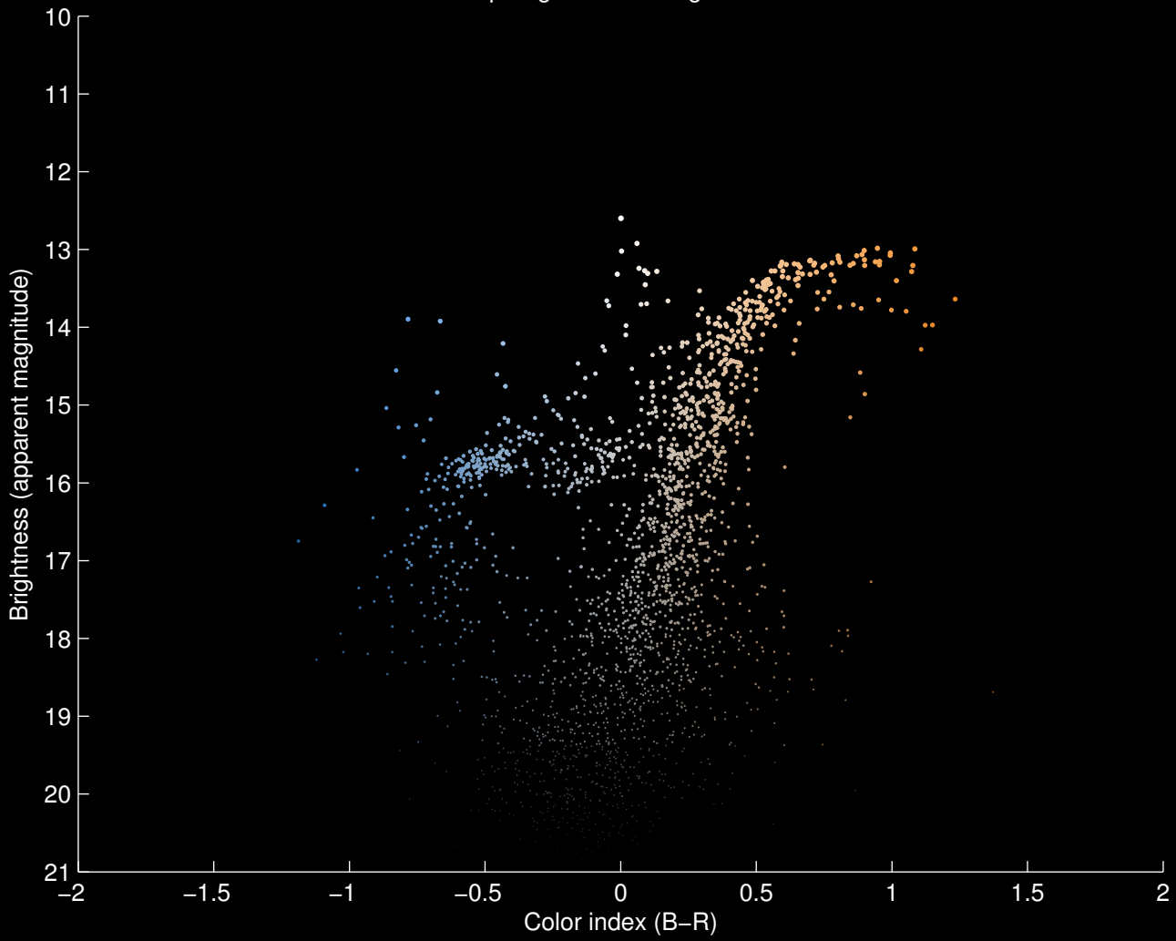
Hertzprung–Russell Diagram for M15
