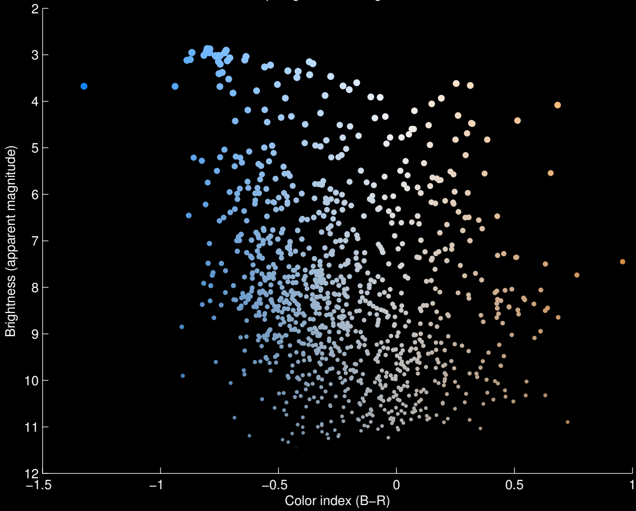
Hertzprung–Russell Diagram for M45
