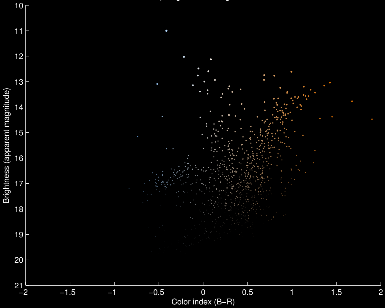
Hertzprung–Russell Diagram for M56
