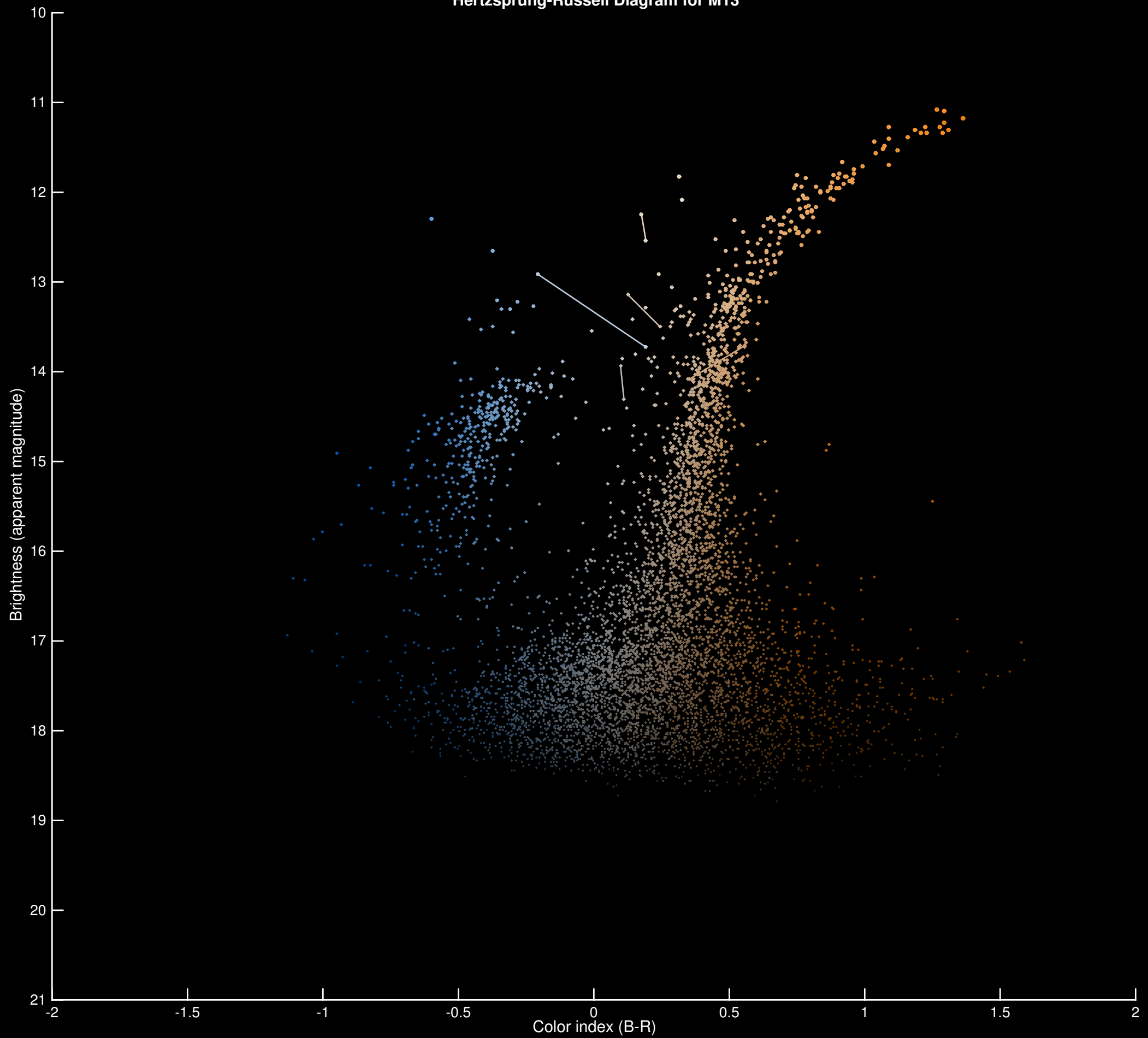
Hertzsprung-Russell Diagram for M13
