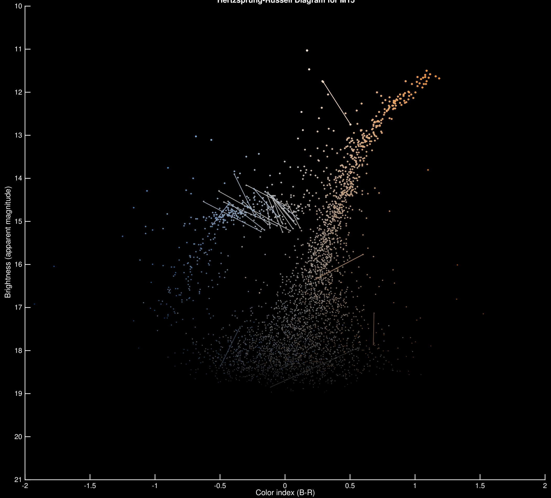
Hertzprung-Russell Diagram for M15
