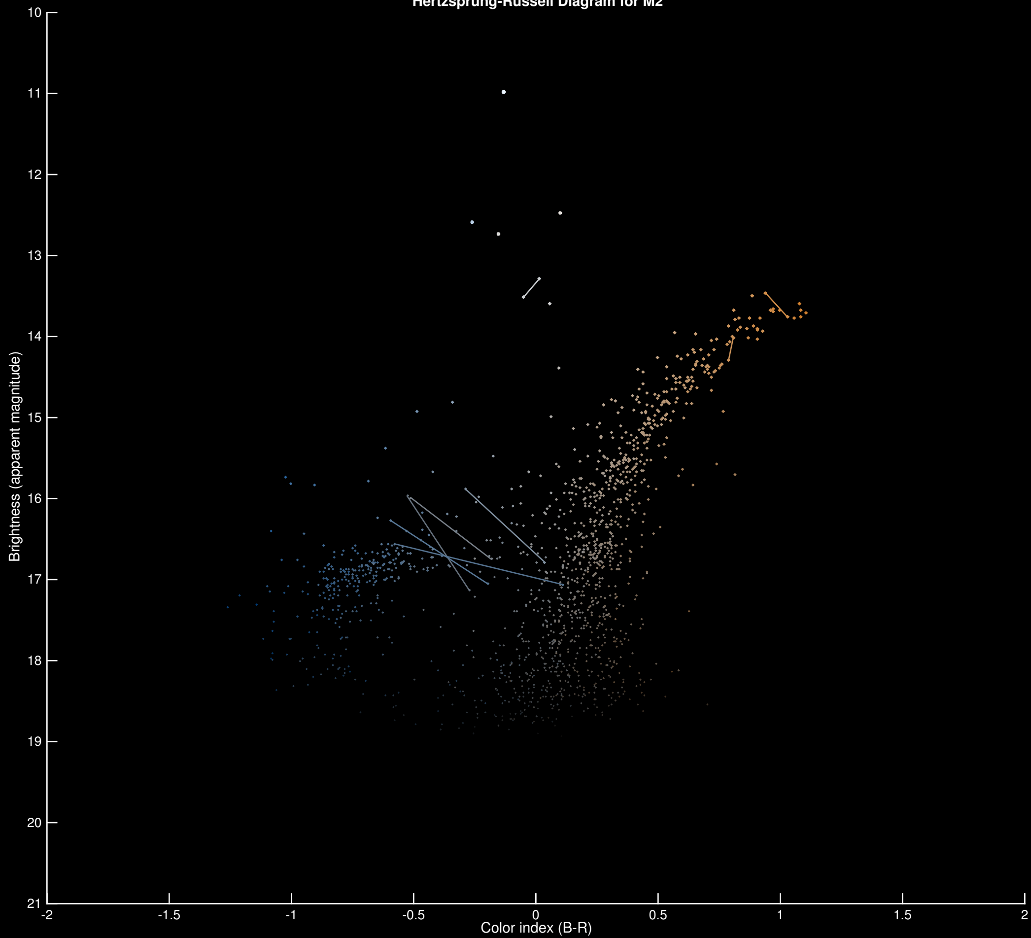
Hertzprung-Russell Diagram for M2
