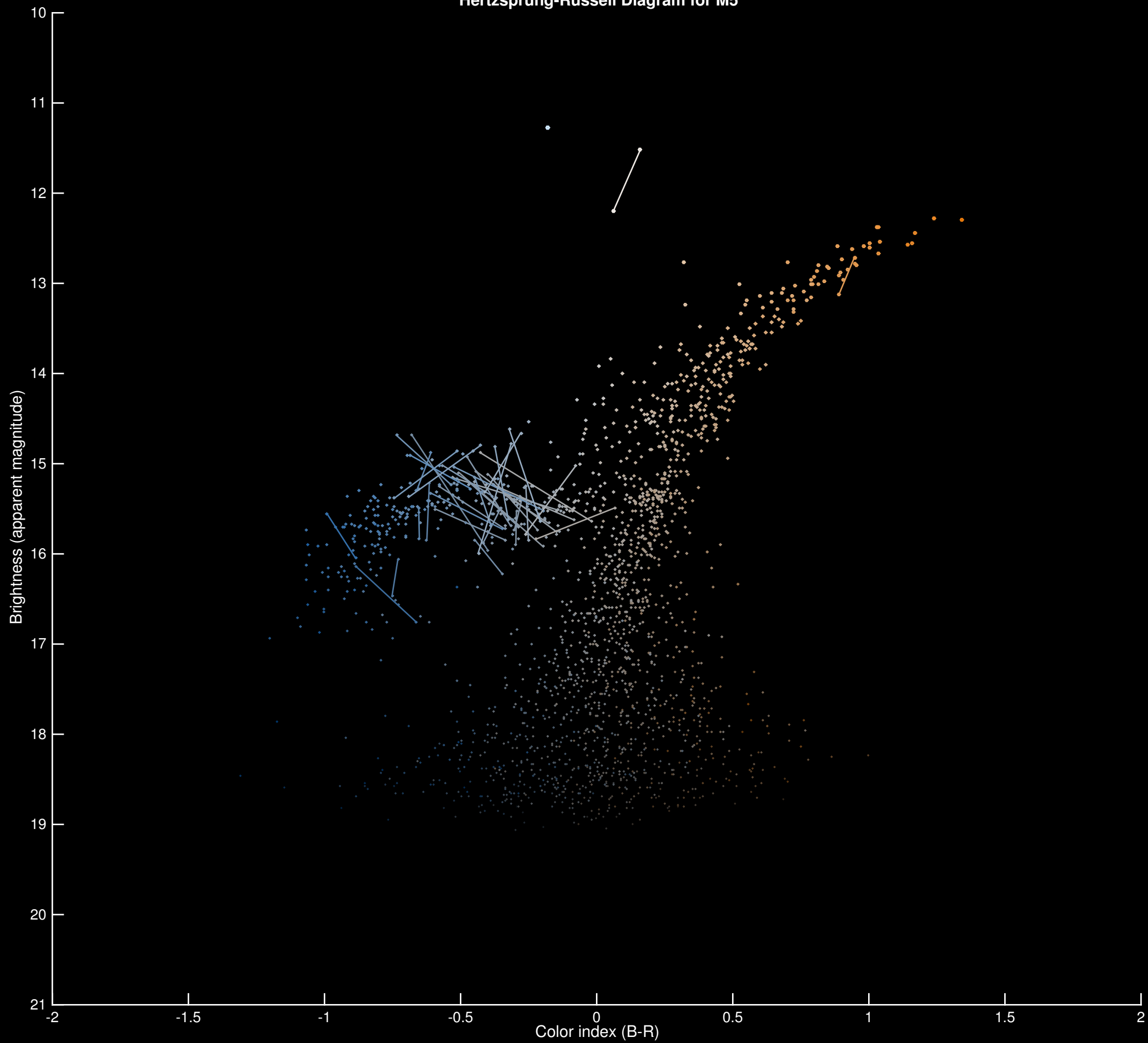
Hertzsprung-Russell Diagram for M5
