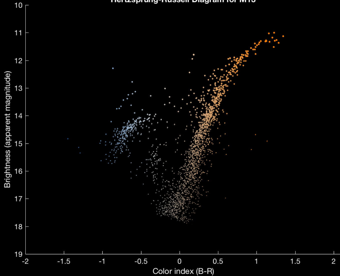
Hertzsprung-Russell Diagram for M13
