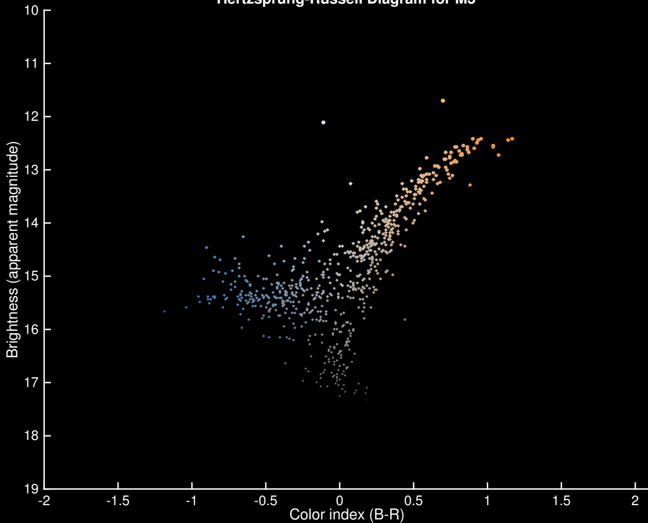
Hertzsprung-Russell Diagram for M3
