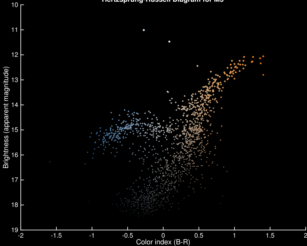
Hertzprung-Russell Diagram for M5
