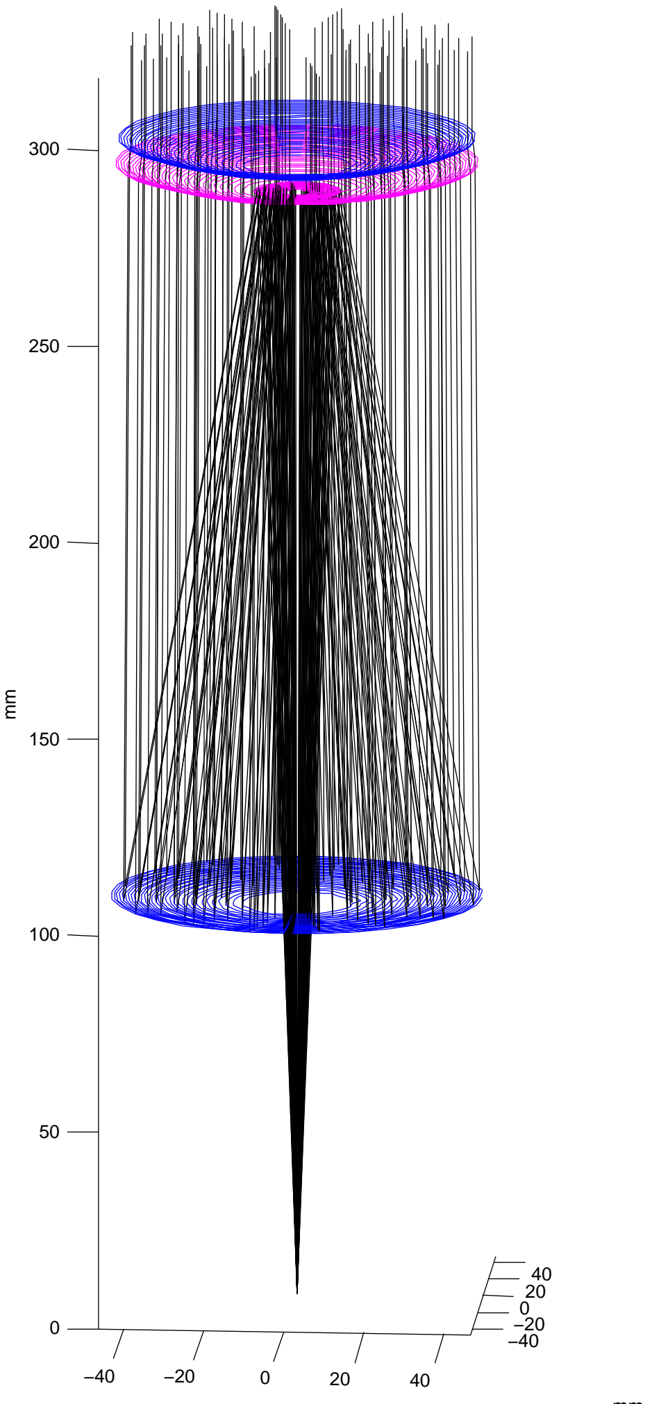
Ray Trace -- On Axis
