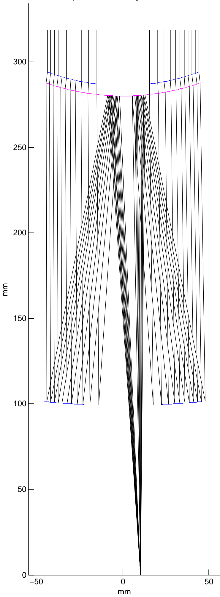
Ray Trace -- 0.5 degrees Off-Axis
