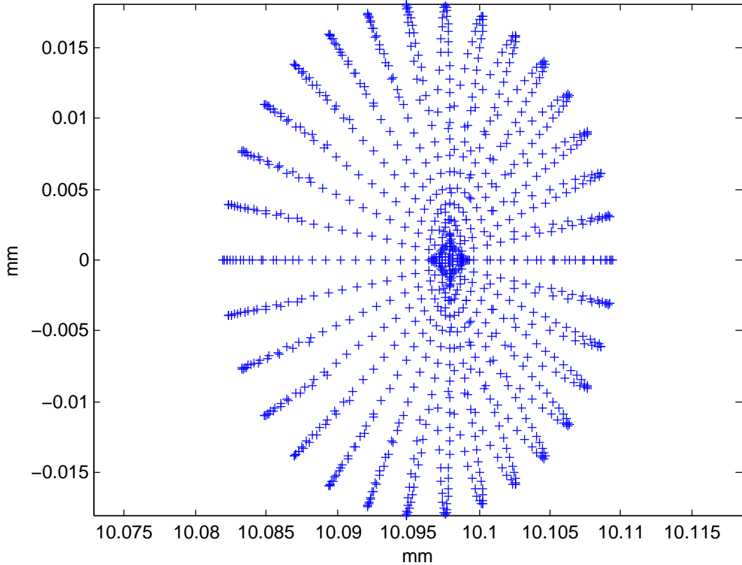
Spot diagram --- 0.5 degrees Off-axis
